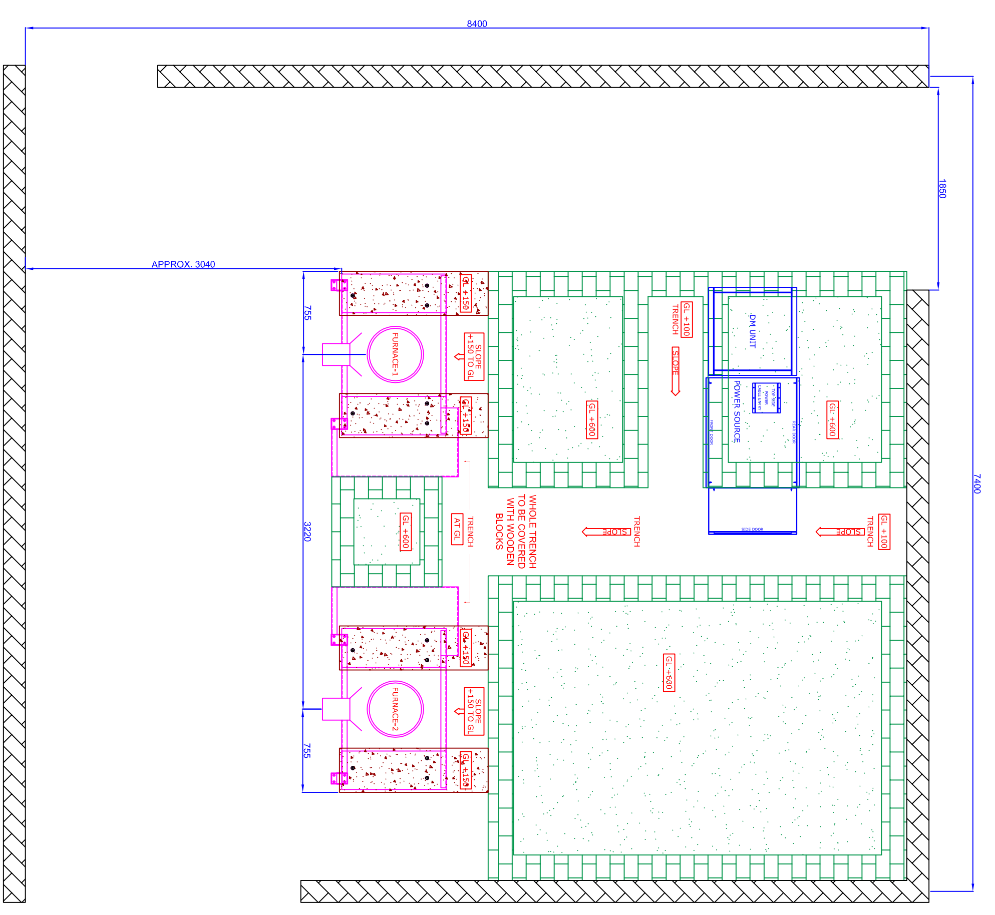
GENERAL ARRANGEMENT
